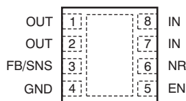
DRB PACKAGE 3mm \times 3mm SON (TOP VIEW)
