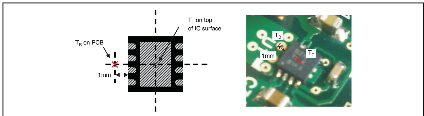
Figure 35. Measuring Points for T_T and T_B
